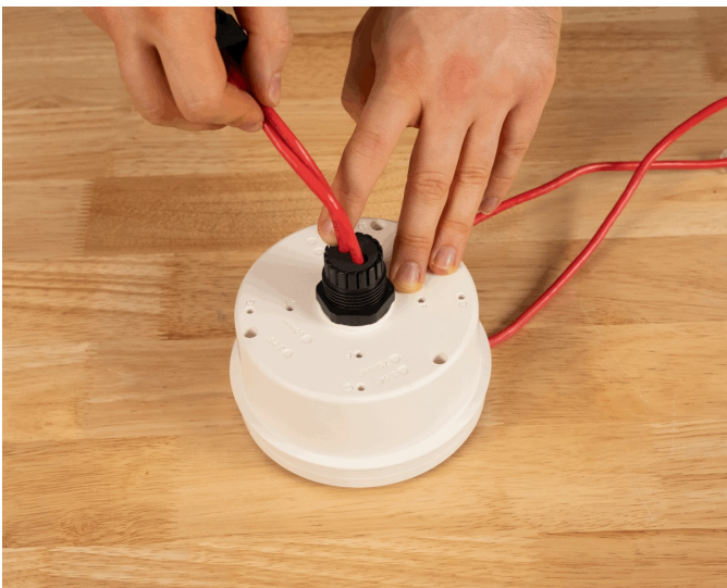
View of seal flush with the gland
